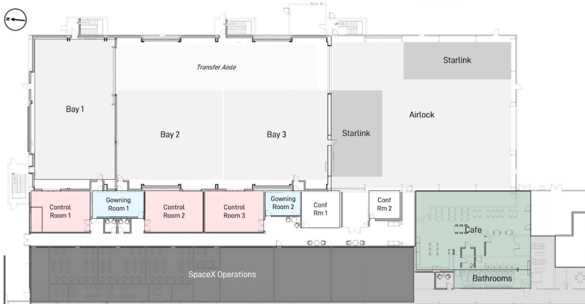
Figure 8-11: Building 398 PPF Layout
